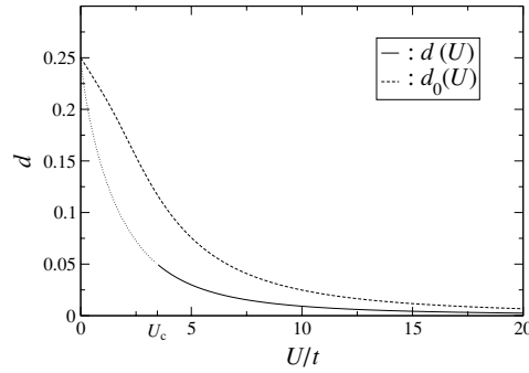
Figure 3. Average double occupancy d_0(U) of the Hubbard model at half band-filling as compared to d(U) (65) for the interacting-electron system with a spin-disordered background.
